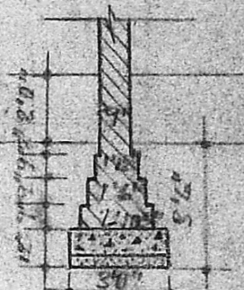
foundation detail scale
