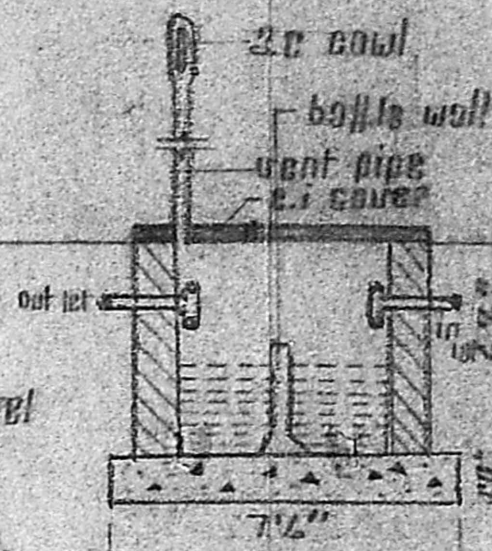
section 7-7
