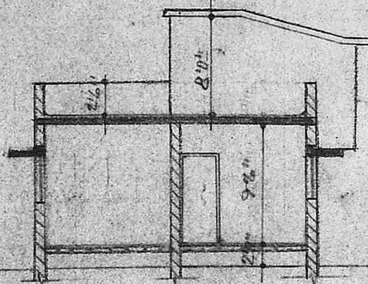
section 2-2
