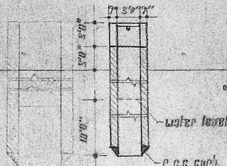
section 6-6
